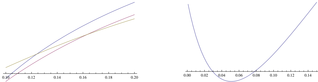
Figure 4: Plots of the maps b \mapsto 1/\mathcal{E}(E_{1,b,c}) over (0.1, 0.2) for c = 0.01, 0.04, 0.08 , and plot of the map c \mapsto 1/\mathcal{E}(E_{1,0.15,c}) over (0, 0.15)
